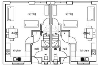
ground floor plans
