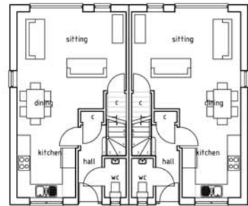
ground floor plans
