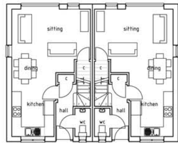
ground floor plans
