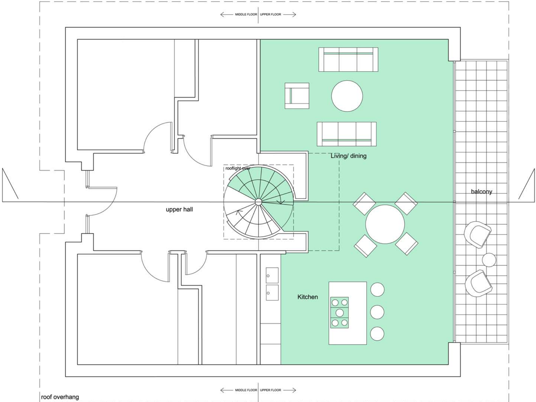
SELF BUILD HOUSES UPPER FLOOR PLAN
